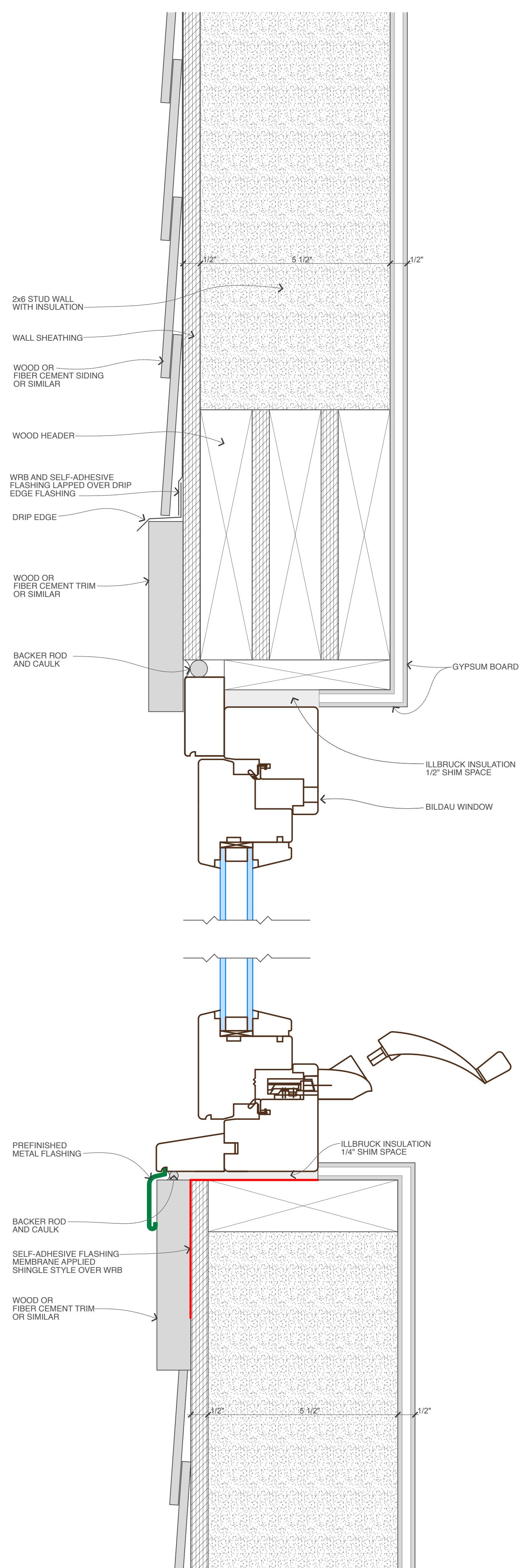
Bildau Crankout Casement Windows Head & Sill Detail
