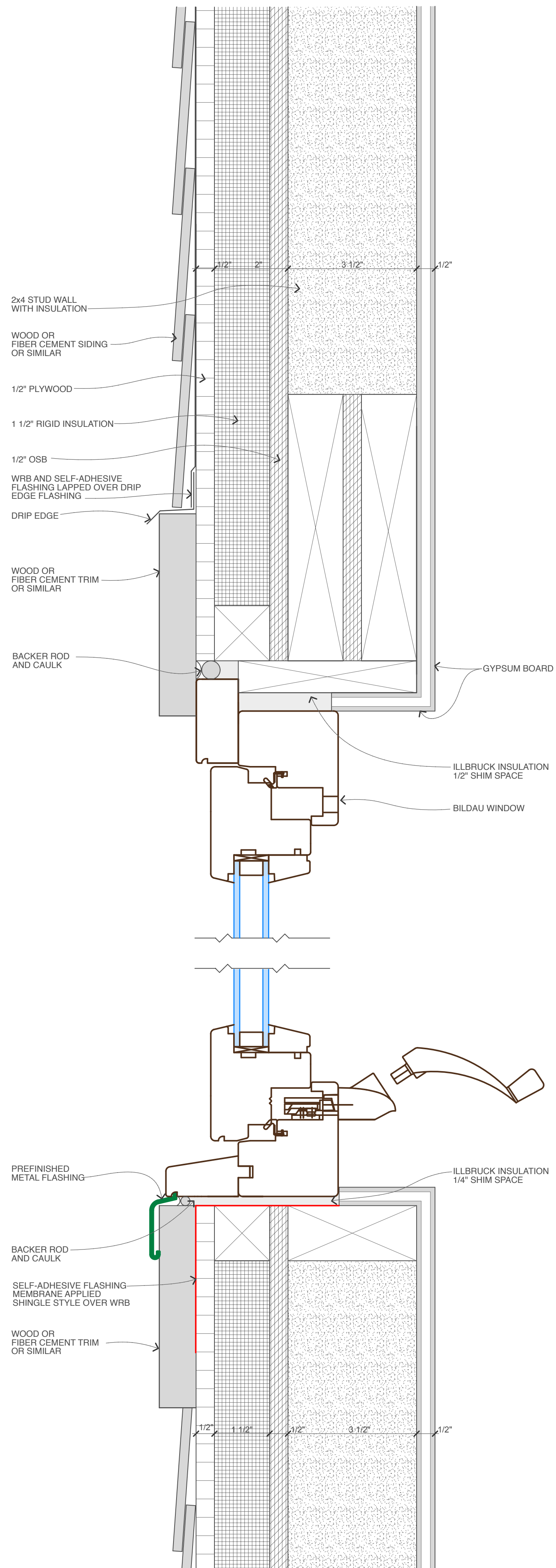
Bildau Crankout Casement Windows Head & Sill Detail
