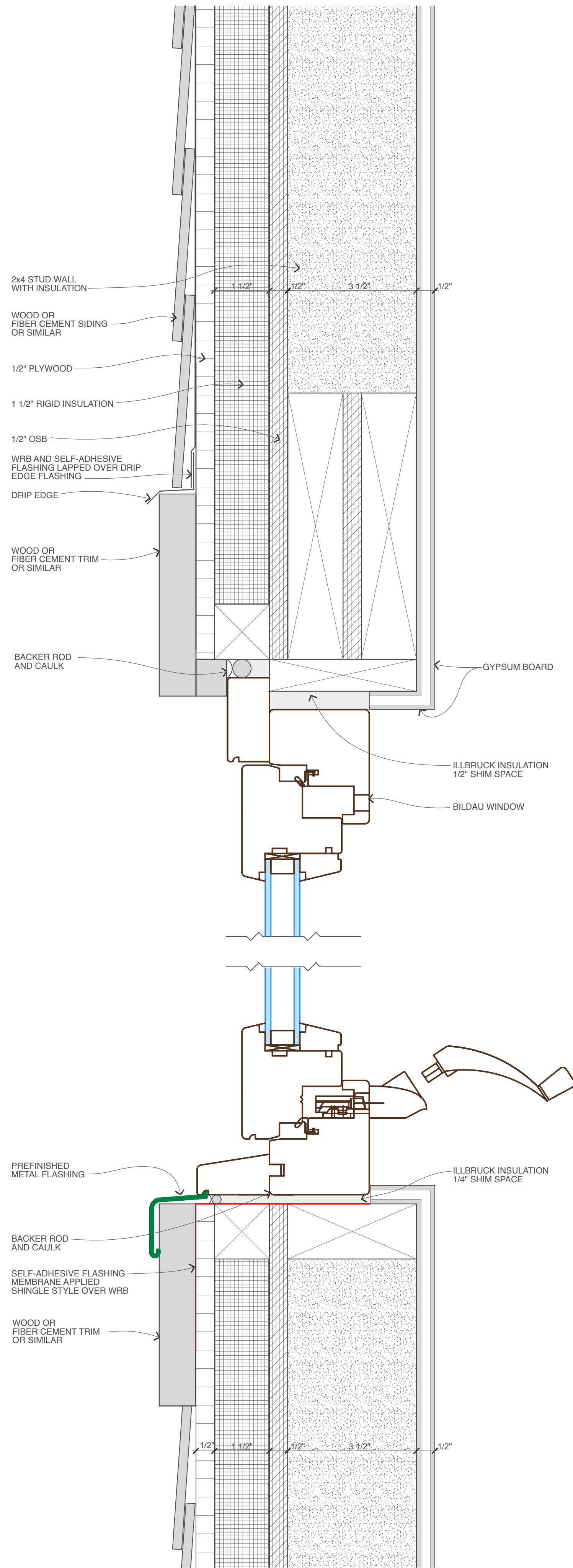
Bildau Crankout Casement Windows Head & Sill Detail
