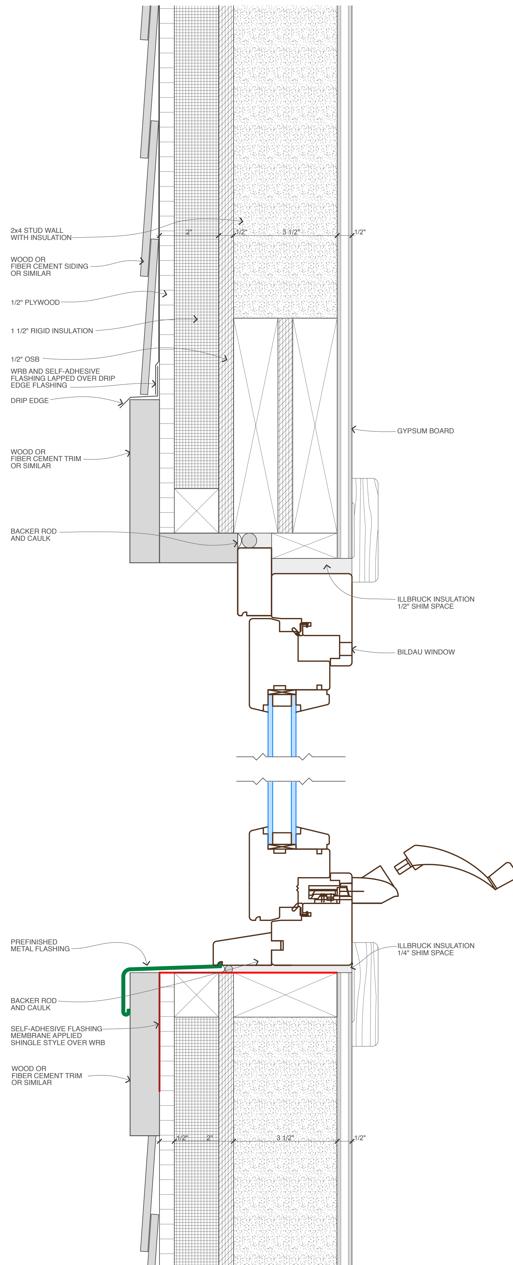
Bildau Crankout Casement Windows Head & Sill Detail
