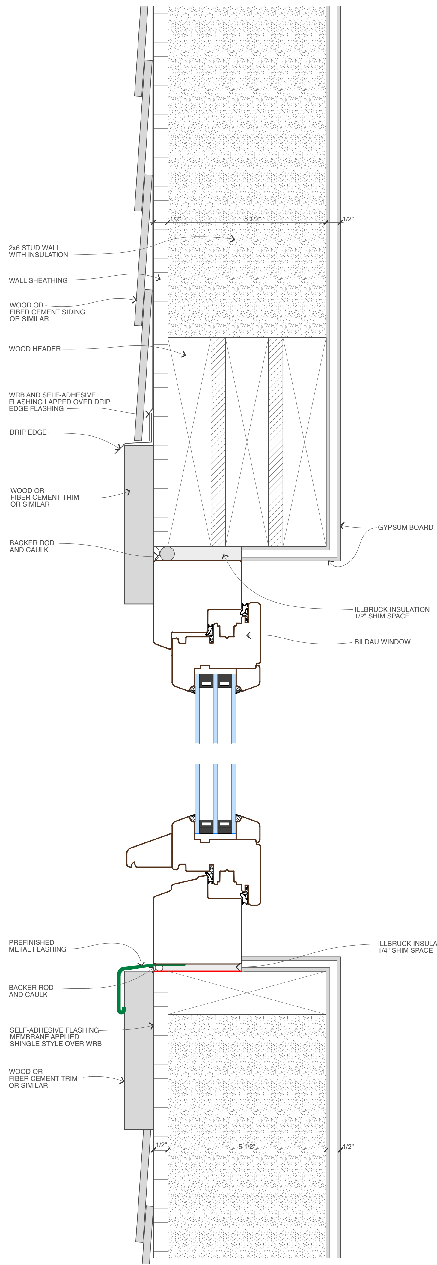
Bildau Windows Historic (inswing) Head & Sill Detail
