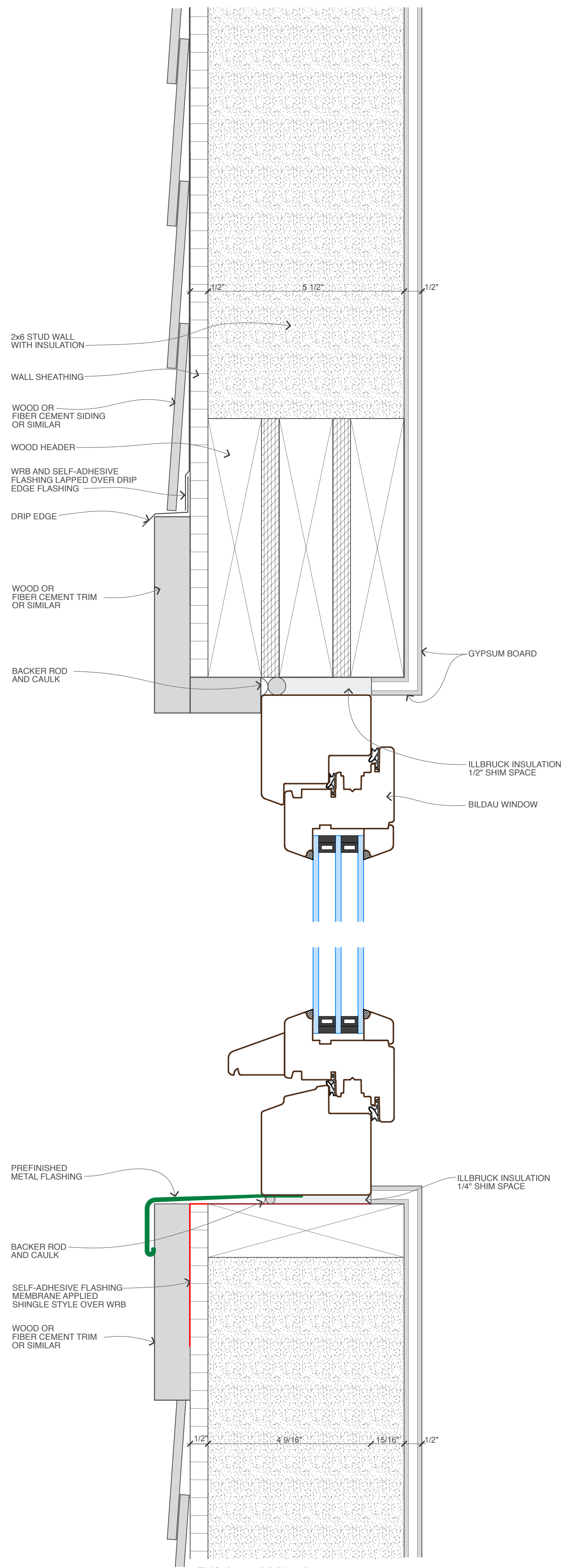
Bildau Windows Historic (inswing) Head & Sill Detail
