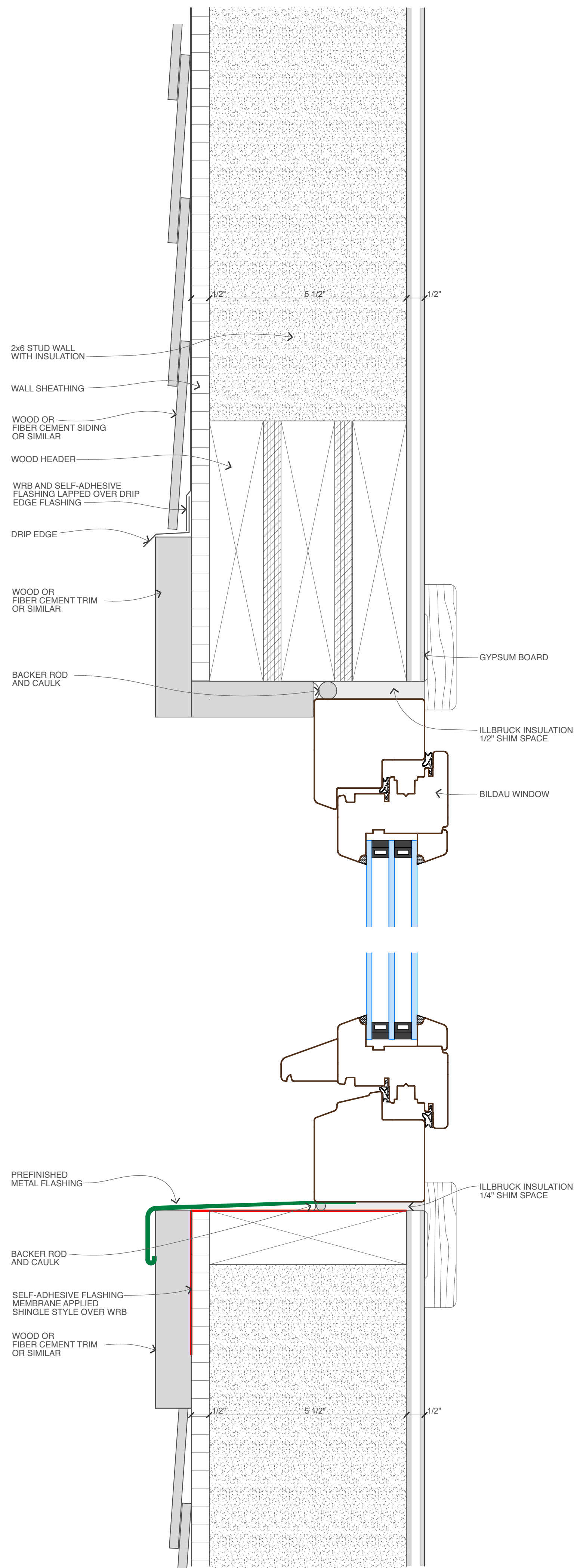
Bildau Windows Historic (inswing) Head & Sill Detail
