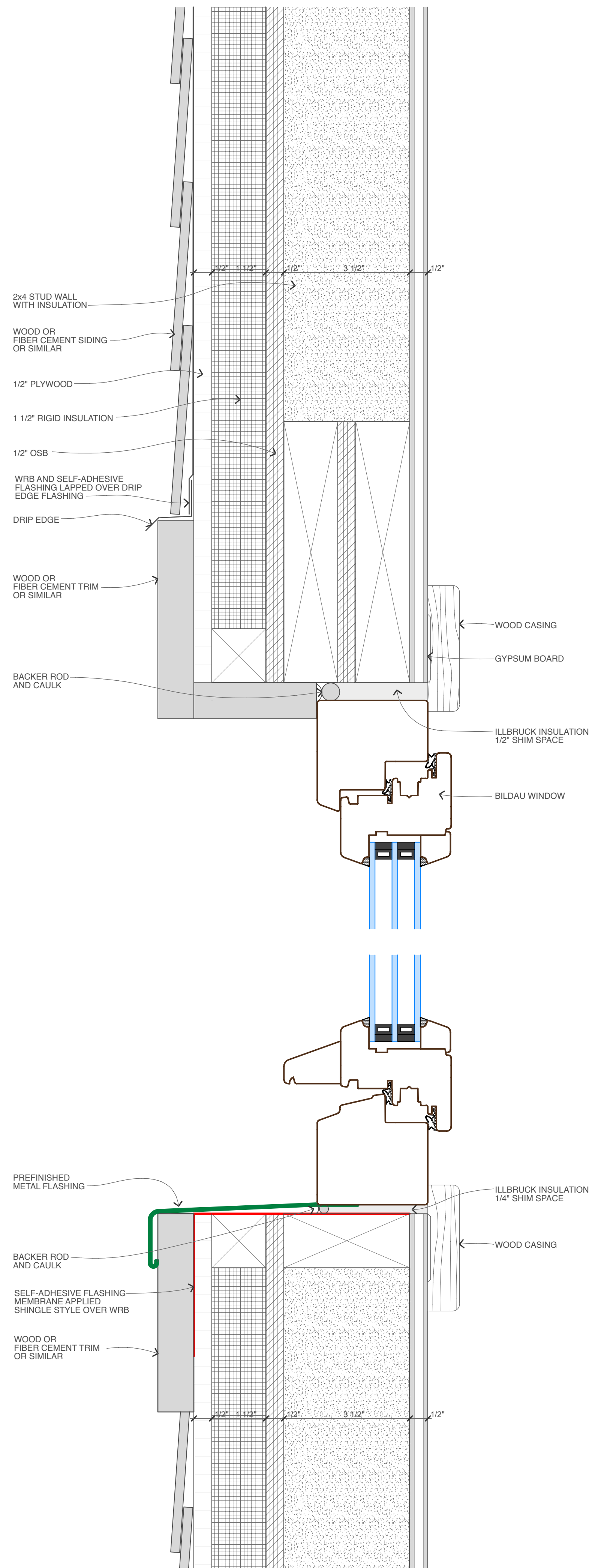
Bildau Windows Historic (inswing) Head & Sill Detail
