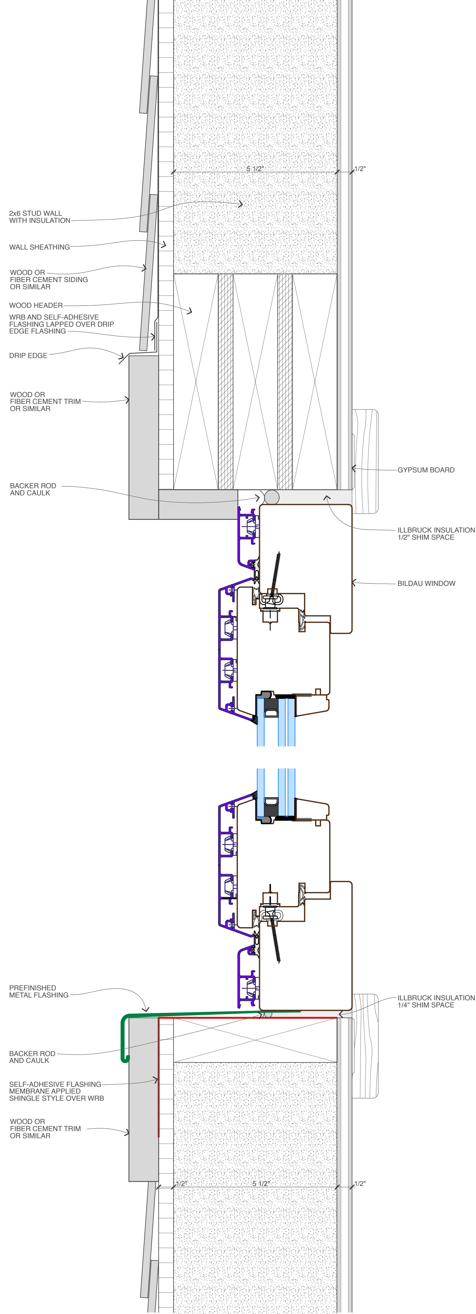
Bildau Windows MIRA Classic Head & Sill Detail
