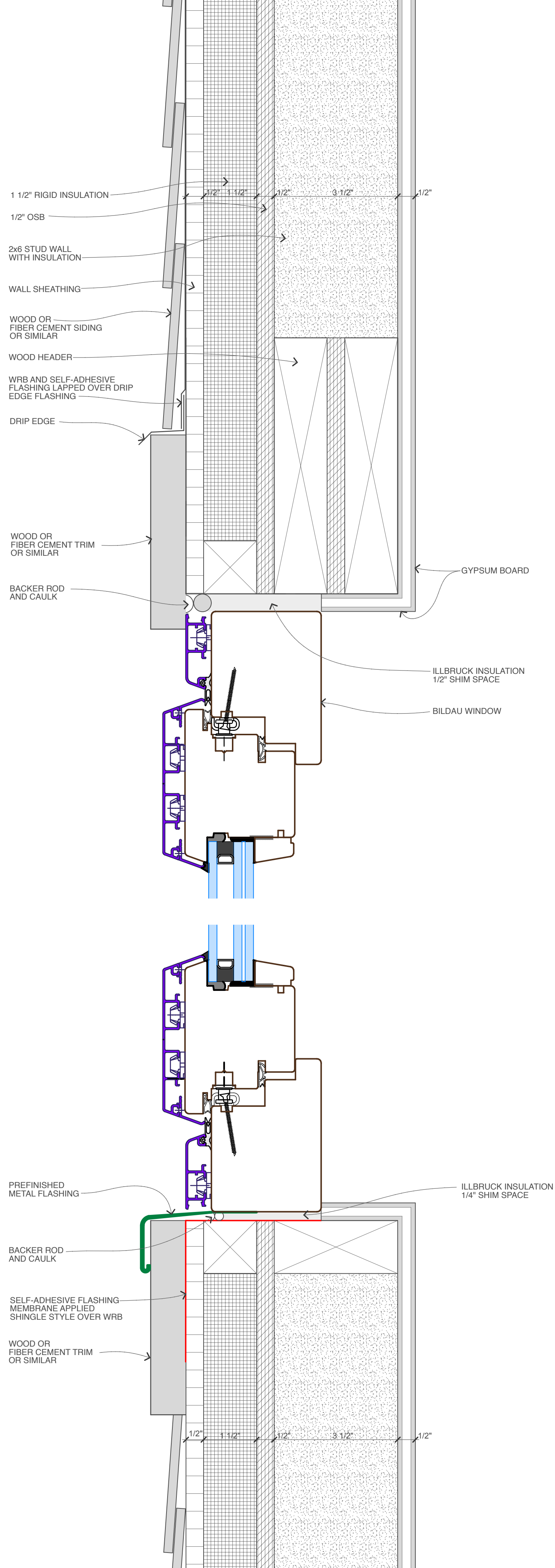
Bildau Windows MIRA Classic Head & Sill Detail
