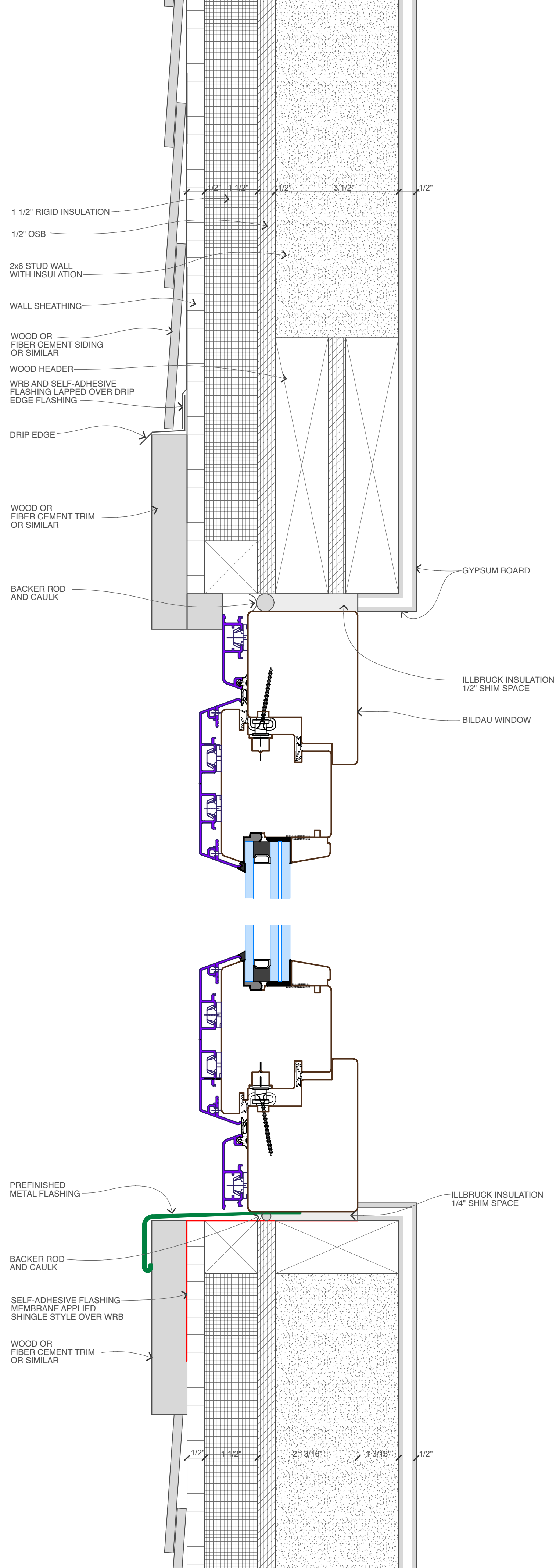
Bildau Windows MIRA Classic Head & Sill Detail
