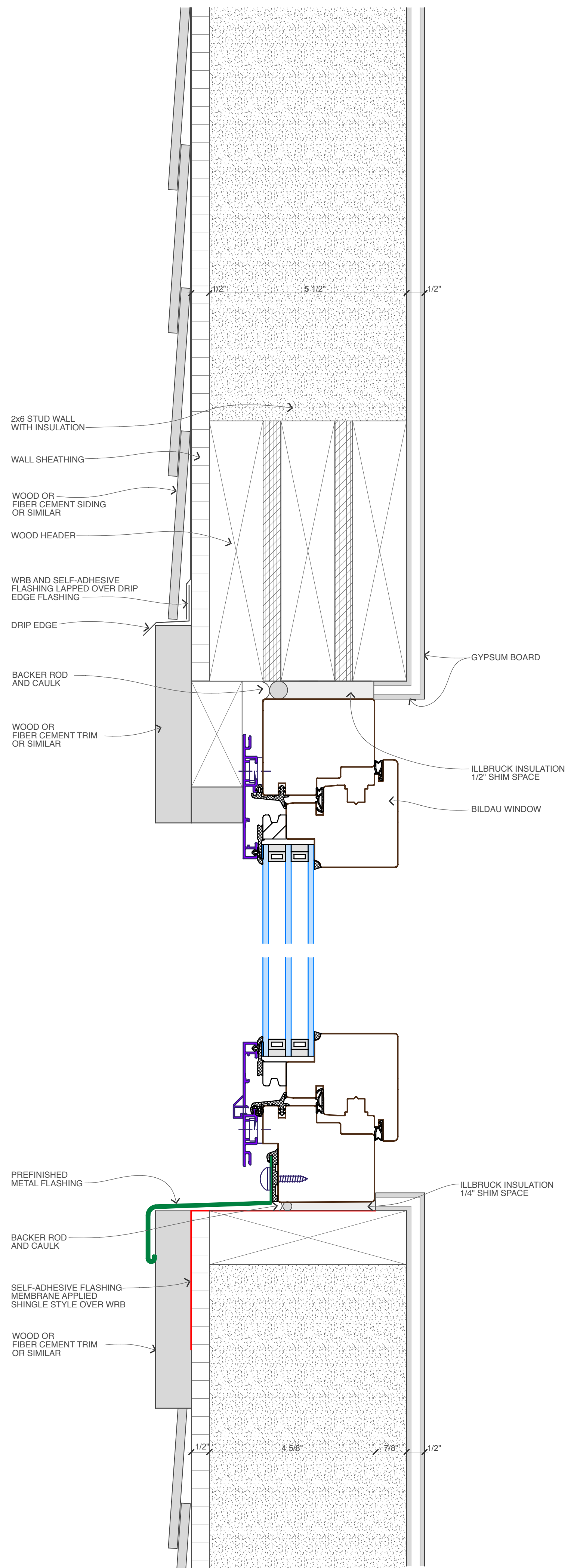
Bildau Windows MIRA Contour Integral (inswing) Head & Sill Detail
