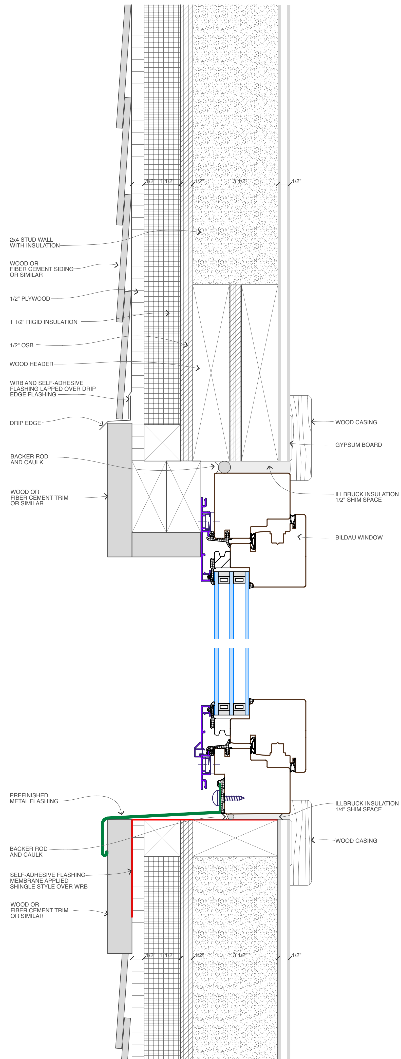
Bildau Windows MIRA Contour Integral (inswing) Head & Sill Detail
