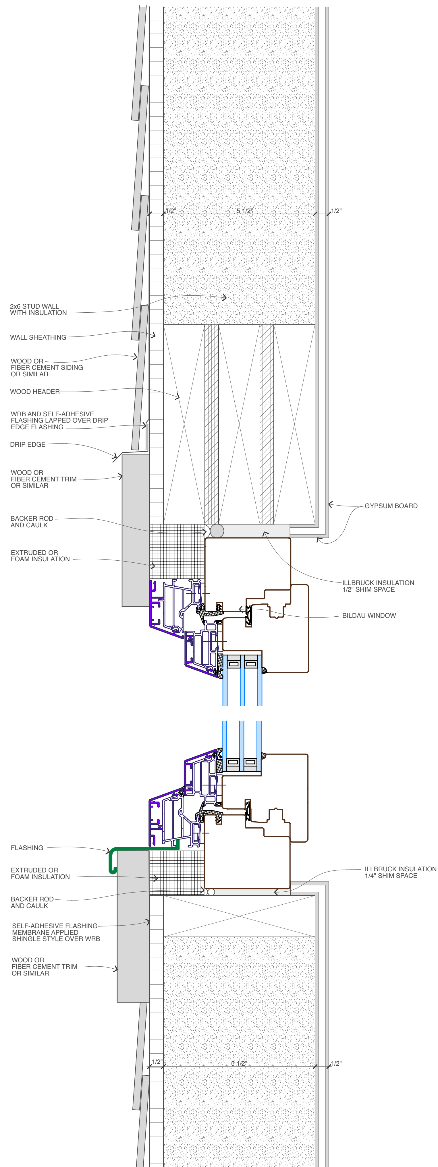
Bildau Windows MIRA Therm (inswing) Head & Sill Detail
