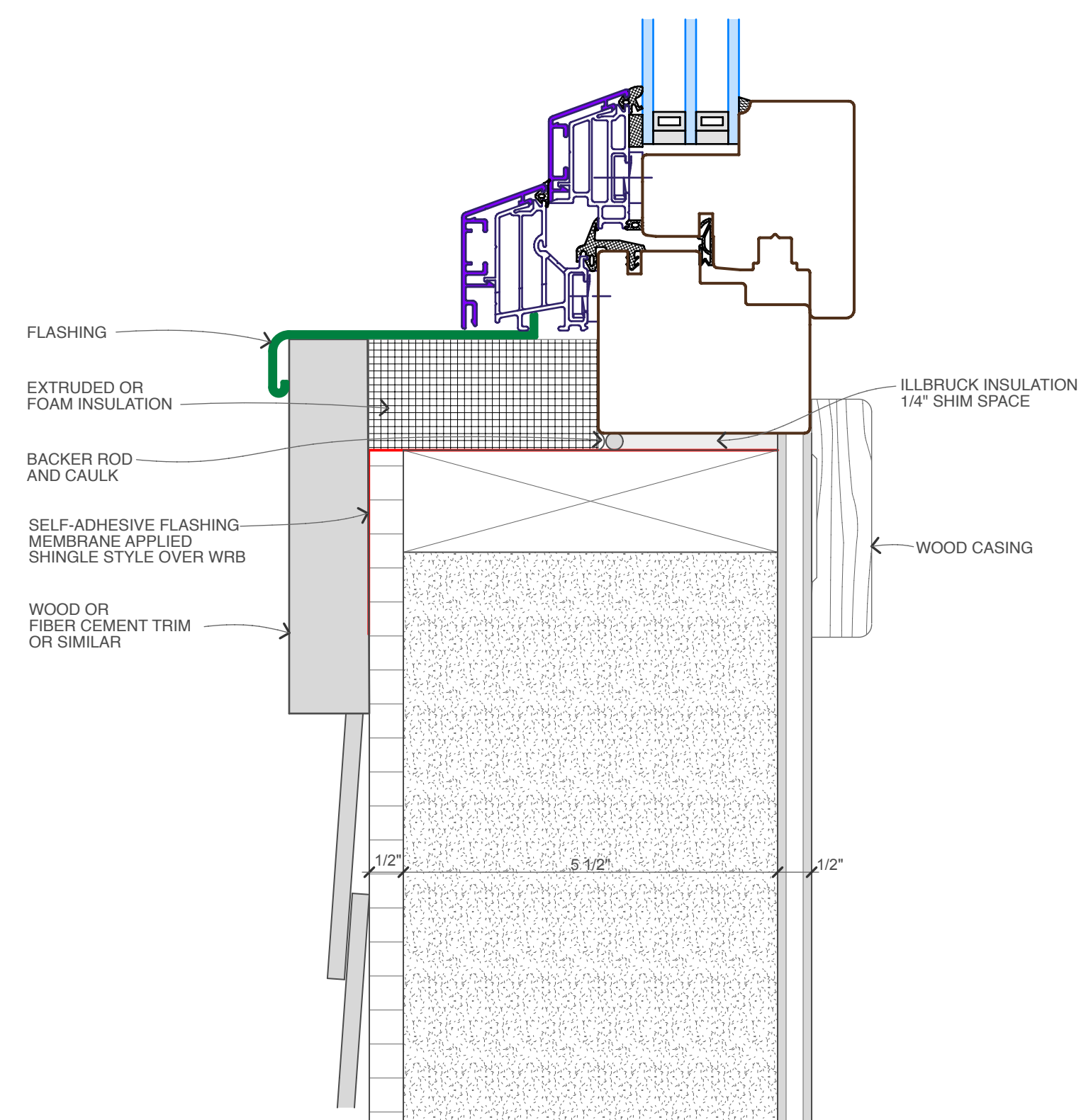
Bildau Windows MIRA Therm (inswing) Head & Sill Detail
