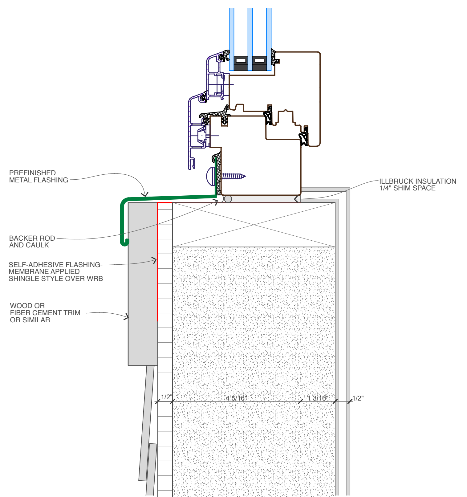
Bildau Windows MIRA (inswing) Head & Sill Detail
