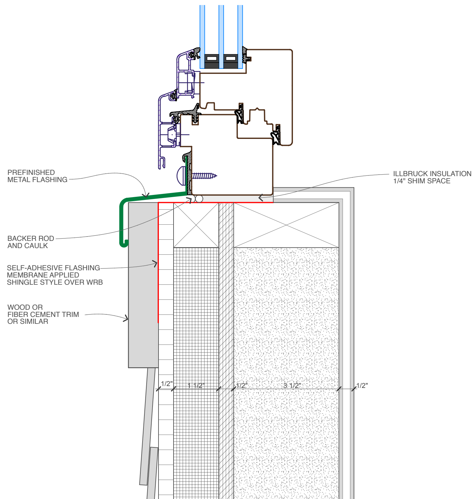
Bildau Windows MIRA (inswing) Head & Sill Detail
