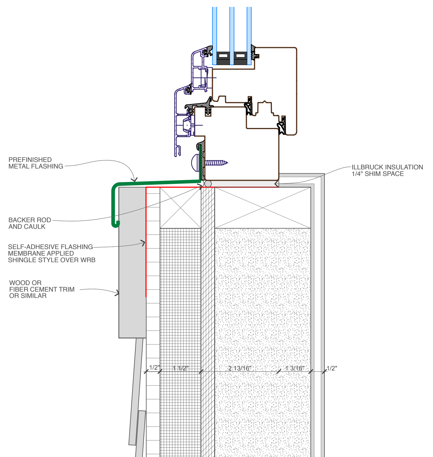
Bildau Windows MIRA (inswing) Head & Sill Detail
