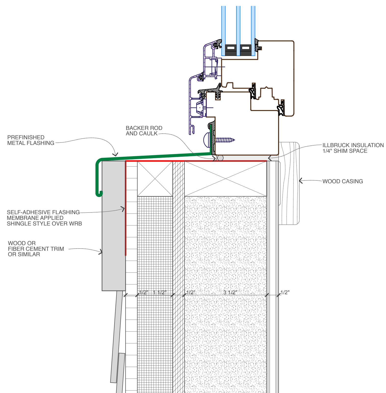
Bildau Windows MIRA (inswing) Head & Sill Detail
